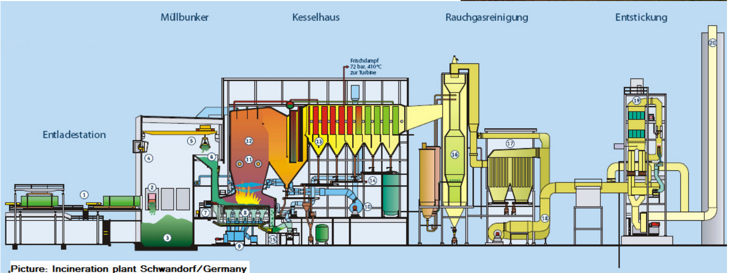
Picture: Incineration plant Schwandorf/Germany
