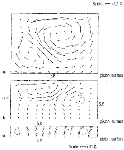
Fig. 7.12 Velocity distributions on compression stroke for the manifold-valve-engine model, 12 \times 12 mesh. (a) X_p^* = 5.63 , CA = 261^\circ , t = 14.5 \text{ msec} = 3970 \Delta t ; (b) X_p^* = 3.56 , CA = 291^\circ , t = 16.2 \text{ msec} = 4250 \Delta t ; (c) X_p^* = 1.0 , CA = 359^\circ , t = 19.9 \text{ msec} = 6300 \Delta t
