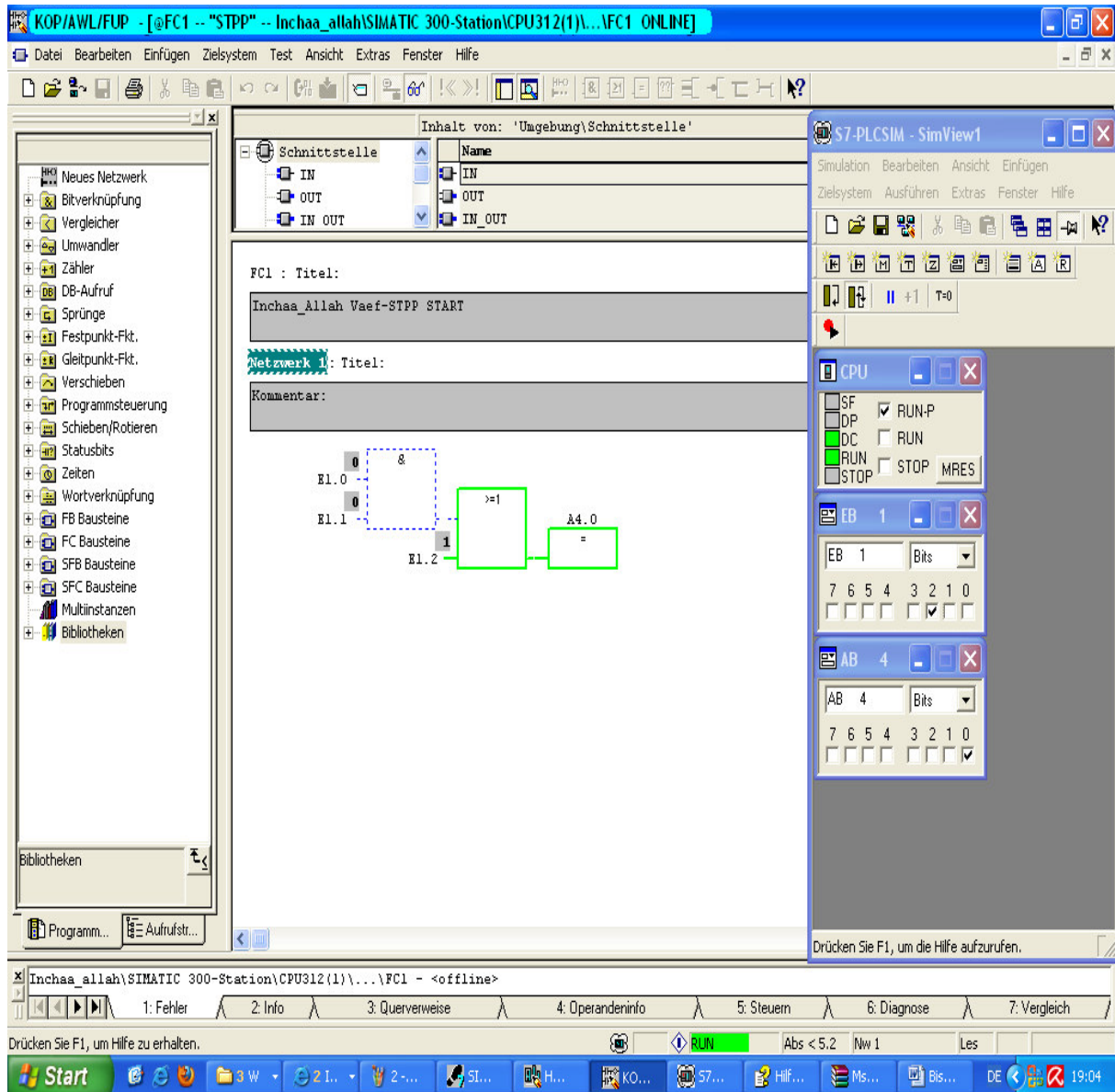
A Small test program
